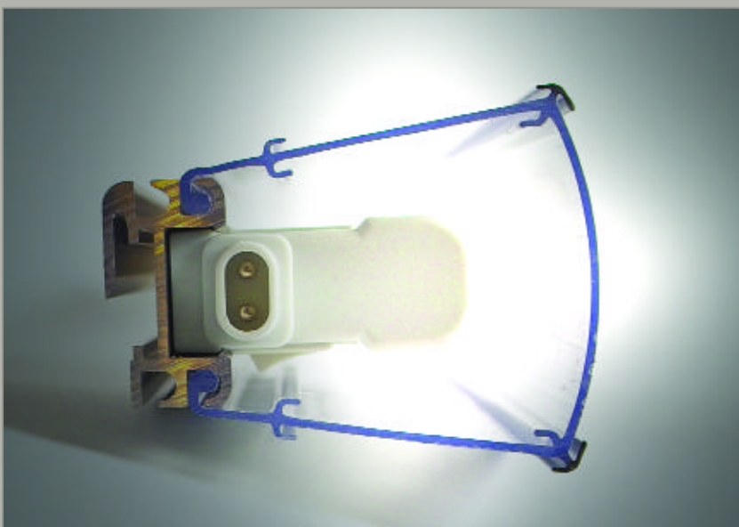
Grooves at the upper and lower side of the chassis offer the possibility of fitting scanner rails.
