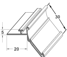
Rail adaptateur T 12, L20mm, rail scanner H30mm, adhésif
