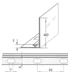
Adapter-T-Profil 11, B21 mm, Kante 40 mm, gelocht
