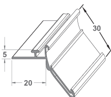
Adapter T-Profile 12, W20, scanner rail H30, self-adhesive
