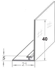
Adapter T-Profile 07, W21, bent 40mm, magnetic
