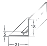
Adapter T-Profile 05, W21, bent 18mm, adhesive
