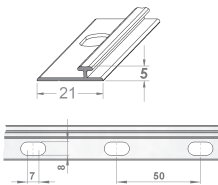
Adapter T-Profile 10, W21, f. wire shelves
