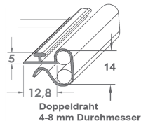
Adapter T-Profile 13, clip for double conductor
