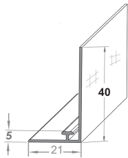
Adapter T-Profile 07, W21, bent 40mm, self-adhesive
