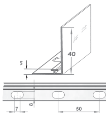
Adapter T-Profile 11, W21, bent up 40mm, f. wire shelves
