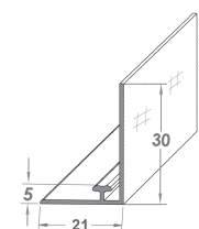
Adapter T-Profile 06, W21, bent 30mm, adhesive
