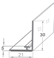
Adapter T-Profile 06, W21, bent 30mm, magnetic
